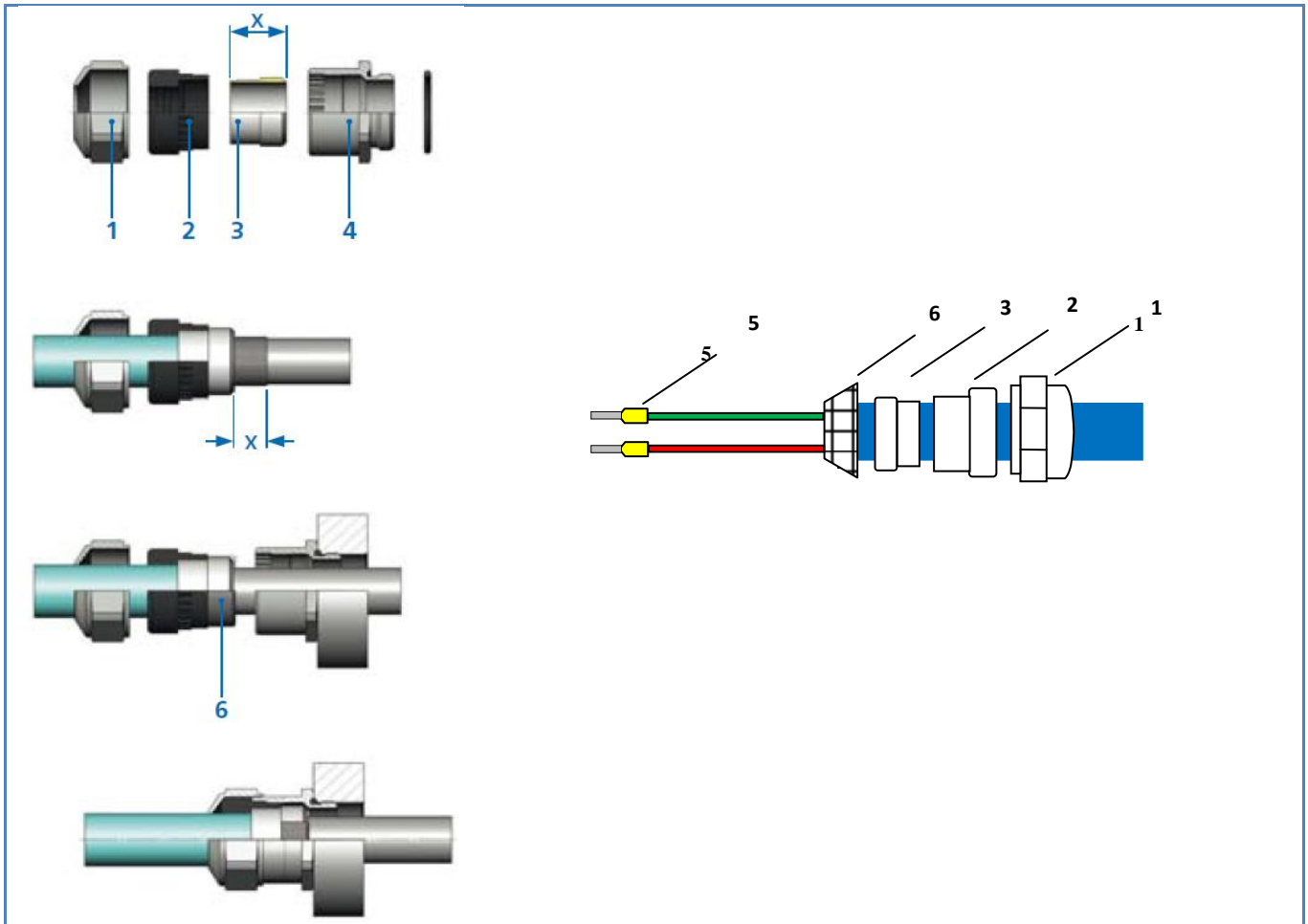
cable gland J-Type
